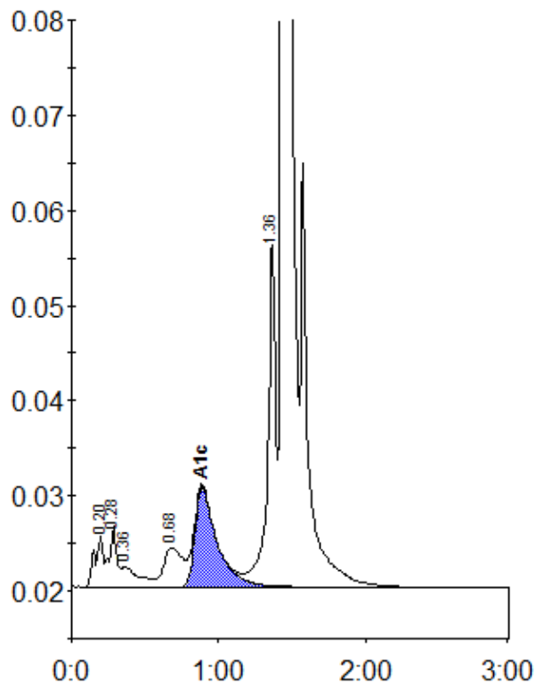
Peak table - ID: 10450830
